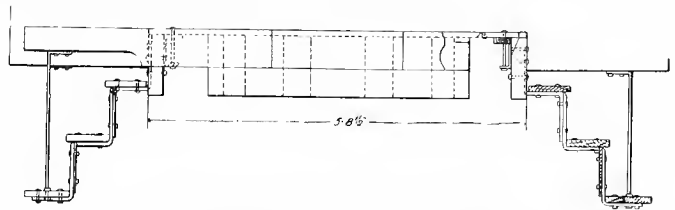
Fig. 1241. Application of Steps and Platform.
